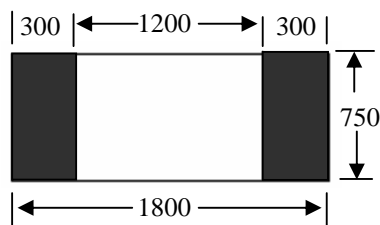
Floor Space Under Bath. All dimension in millimetres
